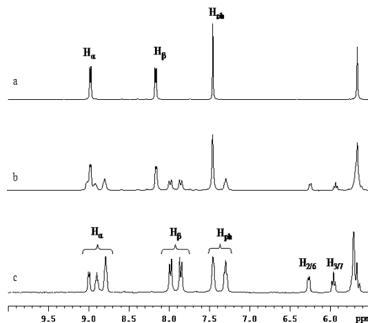
Fig. 1 Partial 1 H NMR spectra recorded in D 2 O/EtOH- d 6 (70 : 30) showing: (a) spectrum of 1 , (b) upon the addition of 0.5 equivalents of 2 , (c) 1 : 1 complex of 1 and 2 . H α , H β and H pn refer to the hydrogens of 1 whereas H 2/6 and H 3/7 refer to the hydrogens of the naphthalene moiety of 2 .
